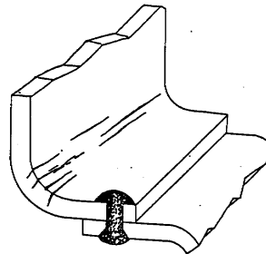
FIGURE 14-3.8(1)--UNSTAYED BOILER FURNACES
