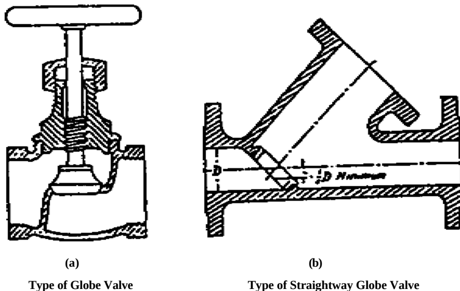
Figure P-43 Typical Globe Valves
