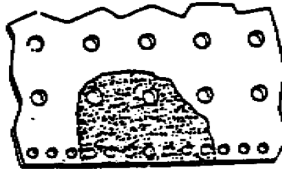
FIGURE 14-3.9(1)--WELD BUILD-UP OF WASTED AREAS
