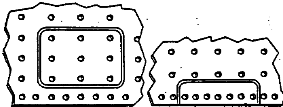
FLUSH PATCHES IN STAYED AREAS
